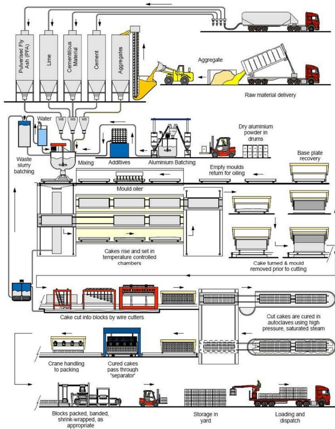
Typical Process Flow Diagram For Autoclaved Aerated Concrete (AAC) Blocks
